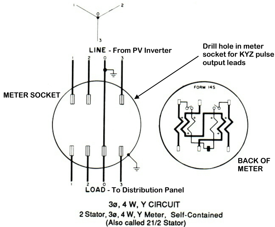
Figure 1. Meter Socket Wiring – 3-Phase 4-Wire Y PV Output
